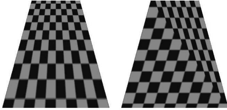
Figure 4.2: Projective space interpolation (left) versus real space interpolation (right). Because the real space interpolation directly references the texture image as it renders, cutting appears between the two polygons. Projective textures compensate for this by using homogeneous texture coordinates. The texture image is indexed after the interpolated coordinates are divided by depth, the homogeneous coordinate. [47]
